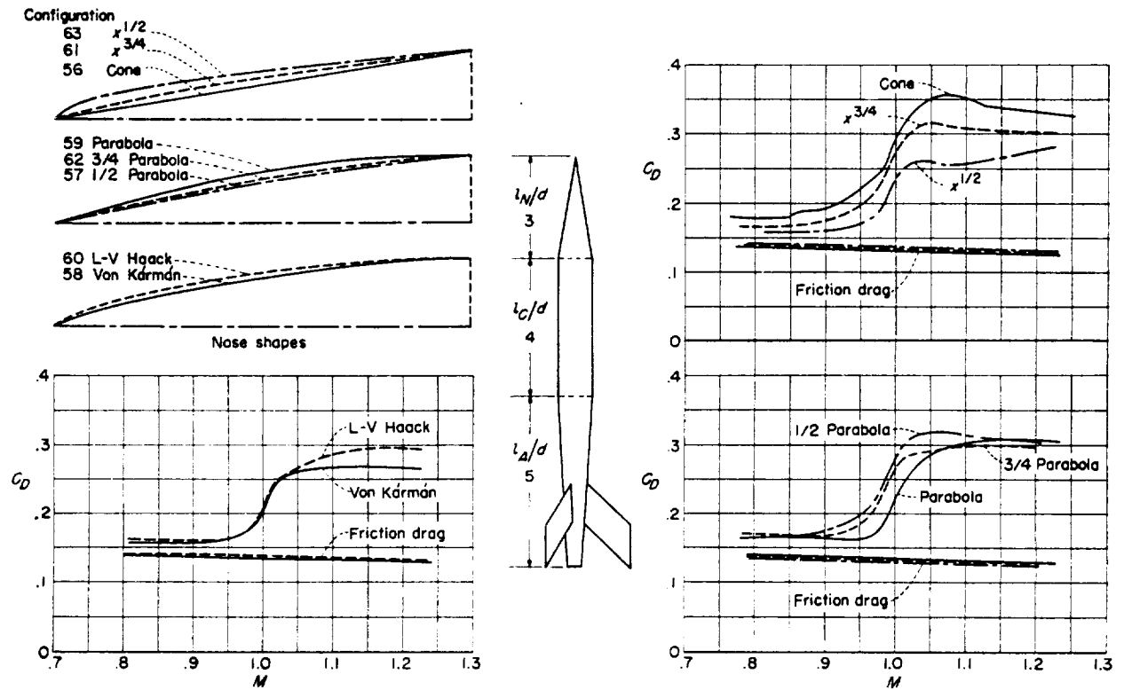
FIGURE 9.—Drag coefficients for eight bodies having fineness-ratio-3 noses of various shapes
