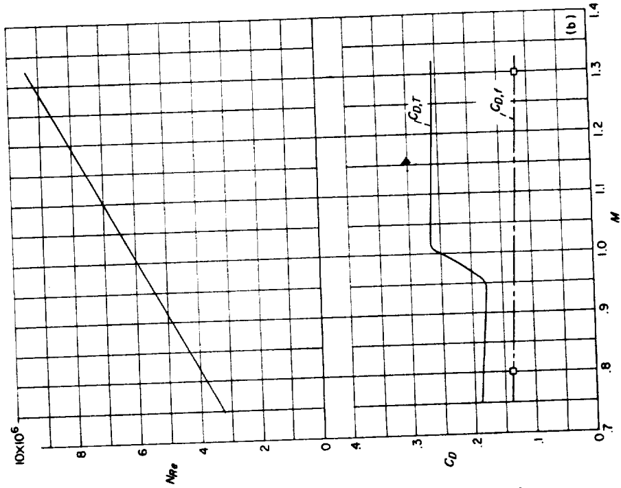
(b) N_{Re} and C_D curves.
