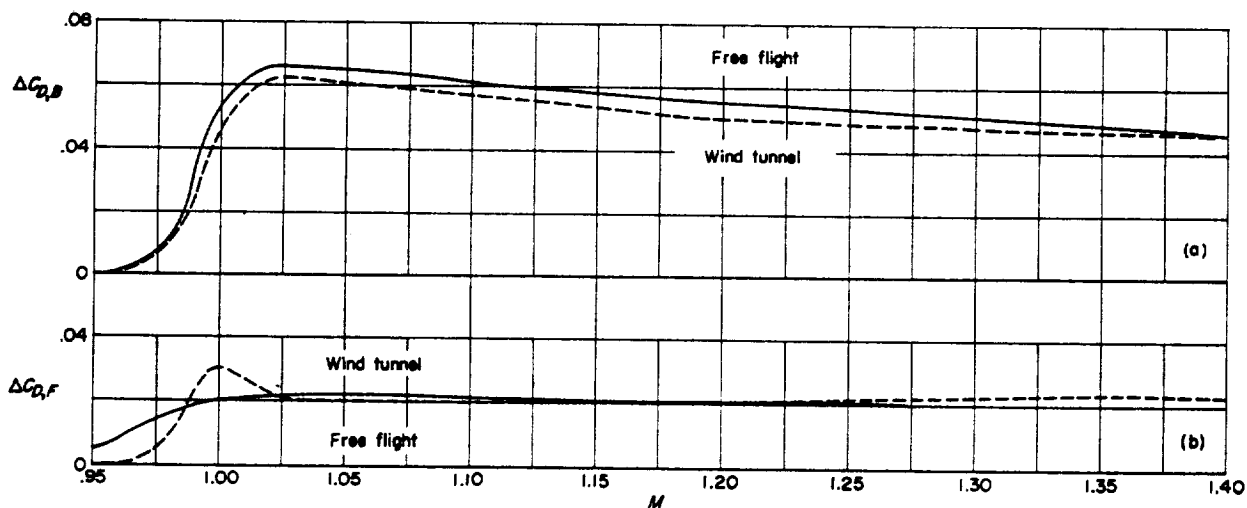
(a) Comparison of drag rise.
